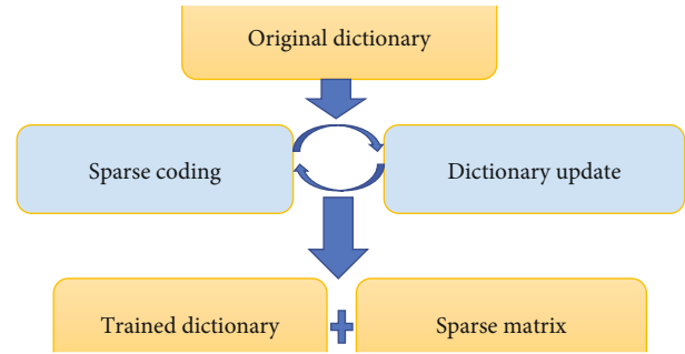
FIGURE 1: The framework of the N-KSVD algorithm.
