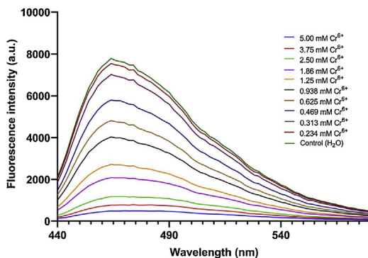
Fig. 2. Emission spectra of the Hydrogel-QCD-composite in the presence of various concentrations of Cr 6+ in river water.
