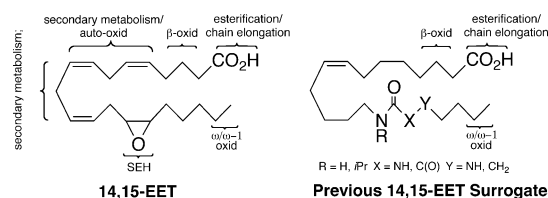
Figure 1. Major routes of metabolism/degradation (oxid = oxidation).
