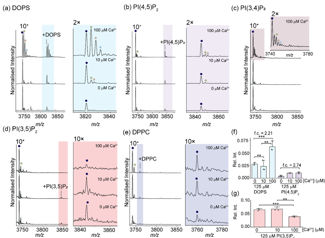
Figure 4. Role of lipids on Ca 2+ binding to Syt-1. (a) (Left) Representative native mass spectra of Syt-1 (12 μM) in the presence of 125 μM DOPS. (Right) magnified view of the Ca 2+ and DOPS binding distribution. (b) (Left) Representative native mass spectra of Syt-1 (12 μM) in the presence of 125 μM PI(4,5)P 2 . (Right) Magnified view of the Ca 2+ and PI(4,5)P 2 binding distribution. (c) Representative native mass spectra of Syt-1 (12 μM) in the presence of 125 μM PI(3,4)P 2 . (Inset) magnified view to show the Ca 2+ binding distribution in the presence of 100 μM Ca 2+ . (d) (Left) Representative native mass spectra of Syt-1 (12 μM) in the presence of 125 μM PI(3,5)P 2 . (Right) Magnified view to show the absence of Ca 2+ and PI(3,5)P 2 binding. (e) (Left) representative native mass spectra of Syt-1 (12 μM) in the presence of 125 μM DPPC. (Right) Magnified view to show the absence of Ca 2+ and DPPC binding. (f) Bar plot of the relative intensities of the Syt-1-lipid-Ca 2+ bound state in the presence of select lipids at different [Ca 2+ ]. f.c. = fold change. (g) Bar plot of the relative intensity of Syt-1-PI(3,5)P 2 at different [Ca 2+ ]. Bars represent the average from n = 3 independent replicates, and error bars represent the standard deviation. * P ≤ 0.05, ** P ≤ 0.01, *** P ≤ 0.001. Deconvoluted mass spectra are shown in Figure S3.
