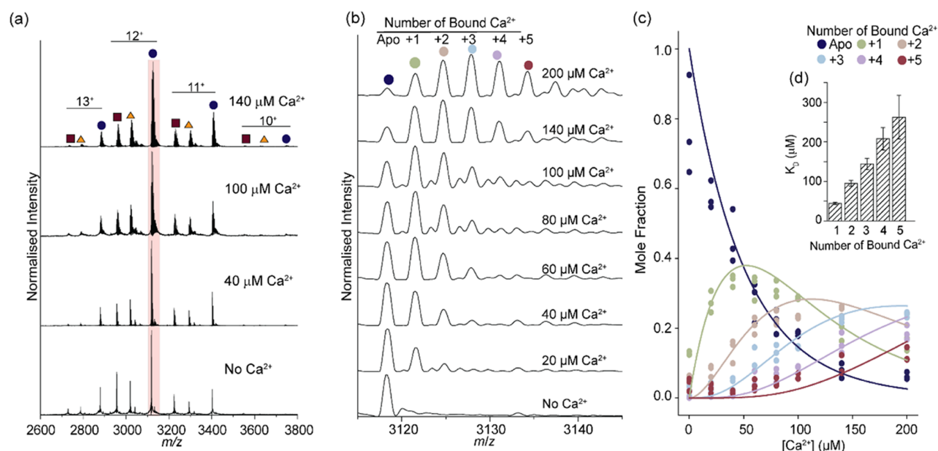
Figure 3. Titration of Ca^{2+} to Syt-1. (a) Stacked native mass spectra at increasing [Ca^{2+}] concentrations following EDTA treatment of Syt-1 (12 \mu M ) to remove endogenous binding. The 12 + charge state is shaded (pink). (b) Representative native mass spectra of the 12 + charge state with increasing [Ca^{2+}] . (c) Plot of mole fraction for each Ca^{2+} -bound state as a function of total [Ca^{2+}] . Solid lines show the fit to an equilibrium binding model to determine the relative binding affinities. Individual measurements from n = 3 independent replicates are shown (colored circles). (d) Bar chart to show magnitude of K_D values for individual Ca^{2+} binding events. K_D values are reported as mean \pm standard deviations, which were derived from an estimated covariance matrix.
