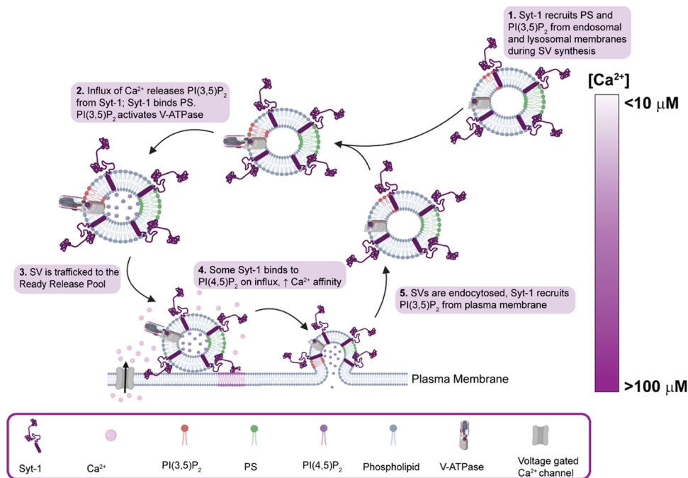
Figure 5. Lipid binding regulates \text{Ca}^{2+} binding to Syt-1. Hypothetical model depicting the key roles of PI(3,5)P 2 and PI(4,5)P 2 binding to Syt-1. PI(3,5)P 2 is sequestered from membranes by Syt-1 for the assembly of V-ATPase in the absence of \text{Ca}^{2+} . Upon influx, PI(3,5)P 2 is released, and PI(4,5)P 2 binds to Syt-1 for the release of neurotransmitters.
