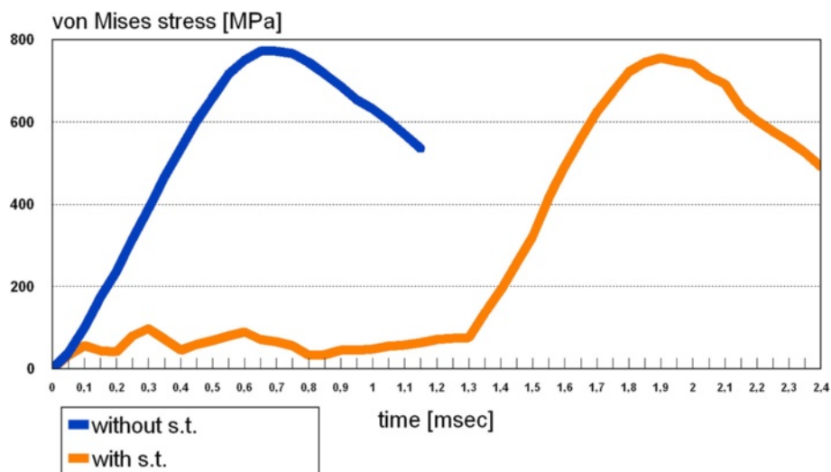
Fig. 8 Comparison of stress curves in the simulation without and with soft tissue (s. t.). The temporal delay caused by simulation of soft tissue is clearly recognizable
