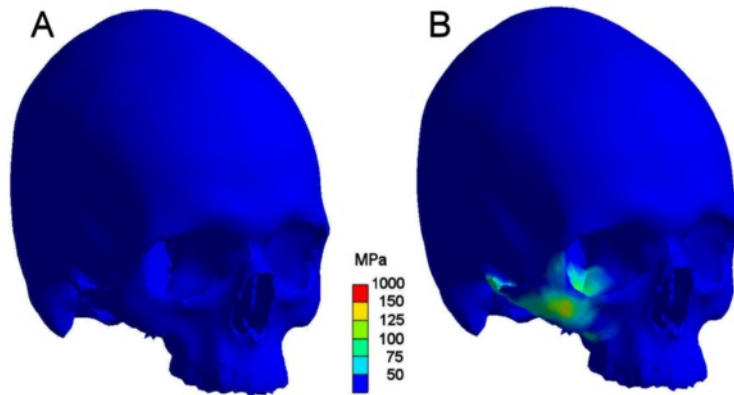
Fig. 7 Situation at 0.15 msec after impact. a: (left skull) scenario with soft tissue simulation; b: (right skull) scenario without soft tissue. Stresses are displayed in megapascal [MPa]. Without facial soft tissue coverage simulation stresses are propagating within the zygoma, whereas no stresses are present in bone with soft tissue simulation at that time
