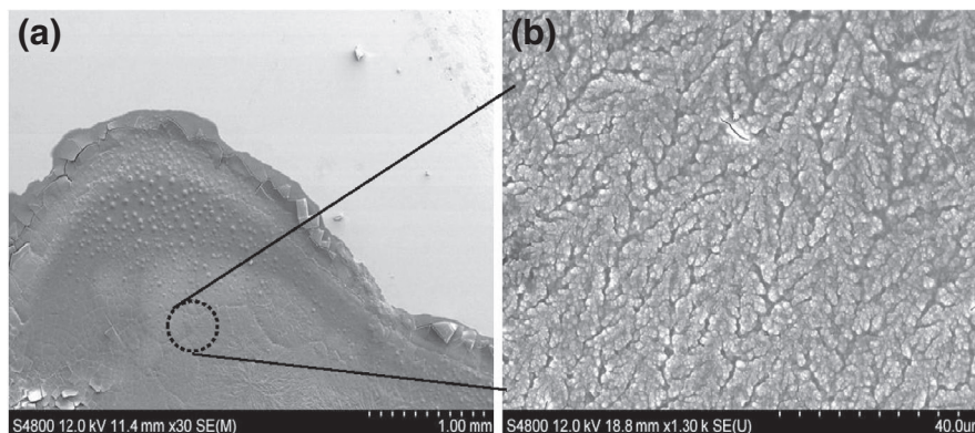
FIGURE 4 Scanning electron microscope images of (a) E. coli (ATCC 8739) on the surface of the Raman substrate at low magnification. (b) A higher magnification image shows a mat of bacteria on the surface where Raman spectra are collected.
