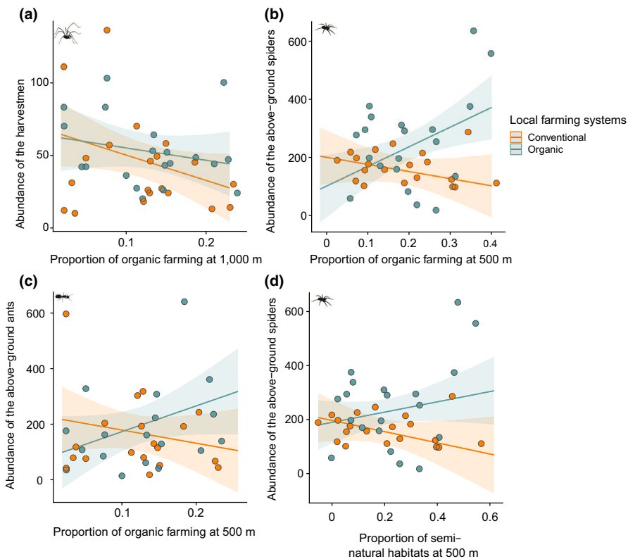
FIGURE 2 Interactive effects of landscape composition and local farming systems on natural enemy abundances. (a) effect of the proportion of organic farming at the 1,000-m scale and local farming systems on harvestman abundance; (b) effect of the proportion of organic farming at the 500-m scale and local farming systems on above-ground spider abundance; (c) effect of the proportion of organic farming at the 500-m scale and local farming systems on the abundance of the above-ground ants; (d) effect of the proportion of semi-natural habitats at the 500-m scale and local farming systems on abundance of the above-ground spiders. R^2 marginal are respectively equal to (a) 0.29, (b) 0.40, (c) 0.20, and (d) 0.40. See also Table 1
