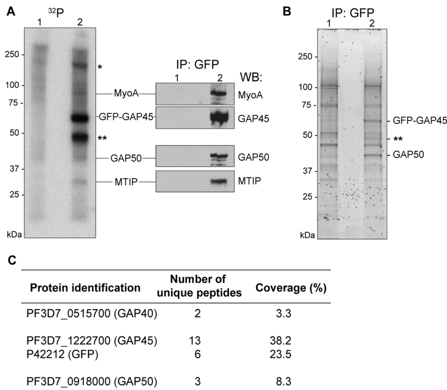
Figure 4. Identification of GAP40 in the P. falciparum glideosome complex. A , wild-type (lane 1) or GAP45-GFP-expressing (lane 2) P. falciparum 3D7 parasites were incubated with radiolabeled phosphate, and proteins binding to a GFP-specific antibody were immunoprecipitated, resolved on an SDS-polyacrylamide gel, and detected by autoradiography. Bands corresponding to two unidentified proteins are labeled with one or two asterisks. In parallel, the same samples were probed with antibodies to known components of the glideosome complex: MyoA, GAP45, GAP50, and MTIP. B , the immunoprecipitation with anti-GFP antibody resin was repeated with unlabeled schizont lysate from wild-type (lane 1) or GAP45-GFP-expressing (lane 2) P. falciparum 3D7 parasites. Immunoprecipitated proteins were fractionated by SDS-PAGE and detected with SYPRO Ruby, and the indicated bands were excised. C , proteins identified in the three excised bands by tryptic digestion and mass spectrometry. The number of unique peptides identified for each protein is indicated, along with the percentage of the protein sequence that these peptides cover. IP , immunoprecipitation; WB , Western blotting.
