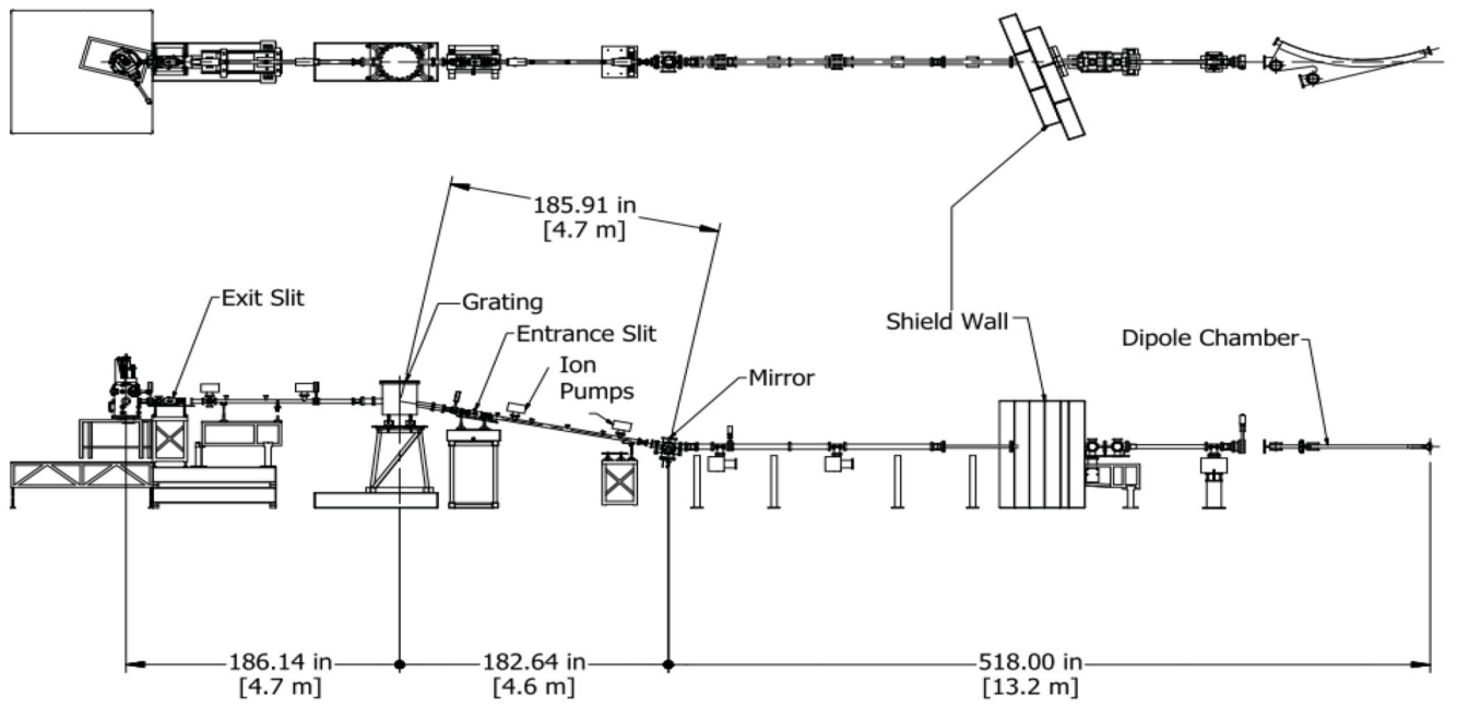
Figure 1. Layout of 5m-TGM beamline at CAMD
