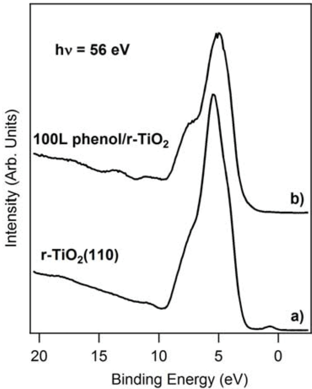
Figure 3. Photoelectron spectra of clean (a) and 100L phenol exposed (b) TiO 2 (110).
