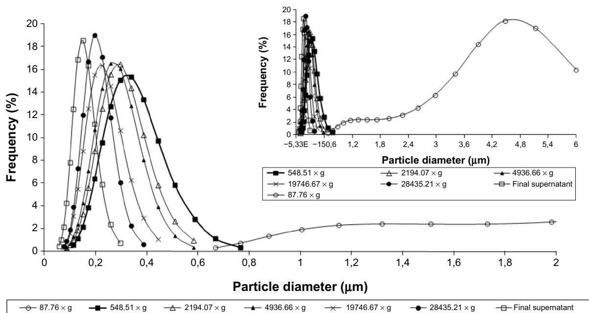
Figure 4 Study of particle separation by centrifugation of NPI. Abbreviation: NP, nanoparticle.
