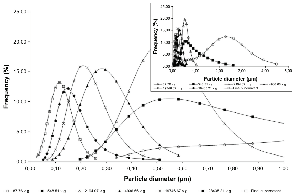
Figure 5 Study of particle separation by centrifugation of NP2. Abbreviation: NP, nanoparticle.
