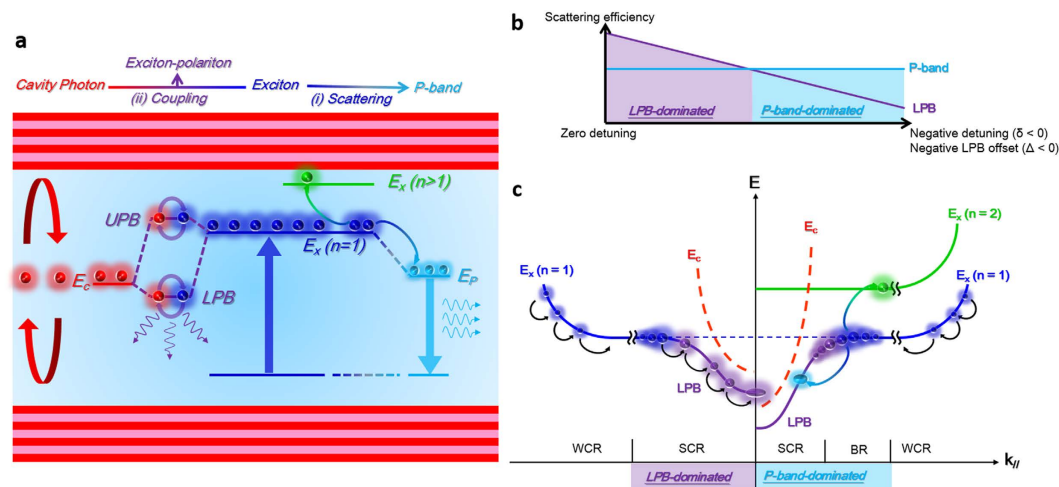
Figure 1. Schematic illustrations of exciton transition channels in a strong coupled ZnO MC. (a) Excitonic-related lasing mechanisms in the strongly coupled ZnO MC. Different states in a strongly coupled ZnO MC including photons (red), ground state excitons (navy blue), higher state excitons (green), exciton-polaritons (blueviolet), and P-band exciton (sky blue) are represented by different colors. The P-band exciton is formed through the X-X scattering such that one of the exciton would scatter to the higher energy state ( n > 1 ) and another one scatters to a lower energy level (P-band) under energy and momentum conservation. (b) Schematic of scattering efficiency trade-off between P-band and polaritons versus the negative detuning and LPB-offset of cavity. The exciton-exciton scattering is independent of the detuning parameter but increases with the exciton density, while the polariton scattering decreases with the detuning parameter. (c) Schematic of the dispersions of a small negatively detuned MC (Left side) and a large negatively detuned MC (Right side). The SCR, WCR and BR indicate the strong coupling region, weak coupling region, and bottleneck region respectively.
