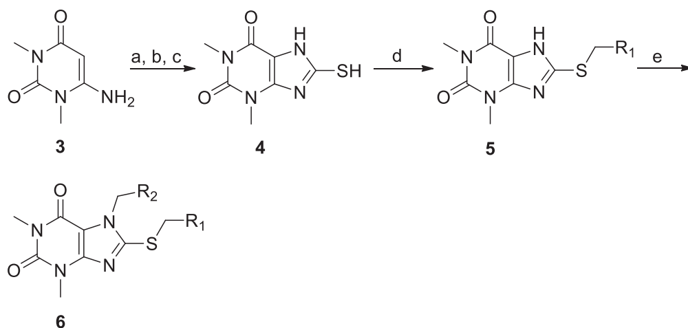
Scheme 2. Preparation of C8-substituted methylxanthine PARGi derivatives 5 and N7, C8-disubstituted methylxanthine PARGi derivatives 6 . Reagents and conditions: (a) NaNO 2 , 50% AcOH, RT, 2 h; (b) Pd/C, H 2 , Ethanol, RT, 2 h; (c) CS 2 , DMF, reflux, 2 h; (d) Alkyl halide, 1% aq. NaOH, RT. (e) alkyl halide, K 2 CO 3 , DMF, 90 °C, 12 h.
