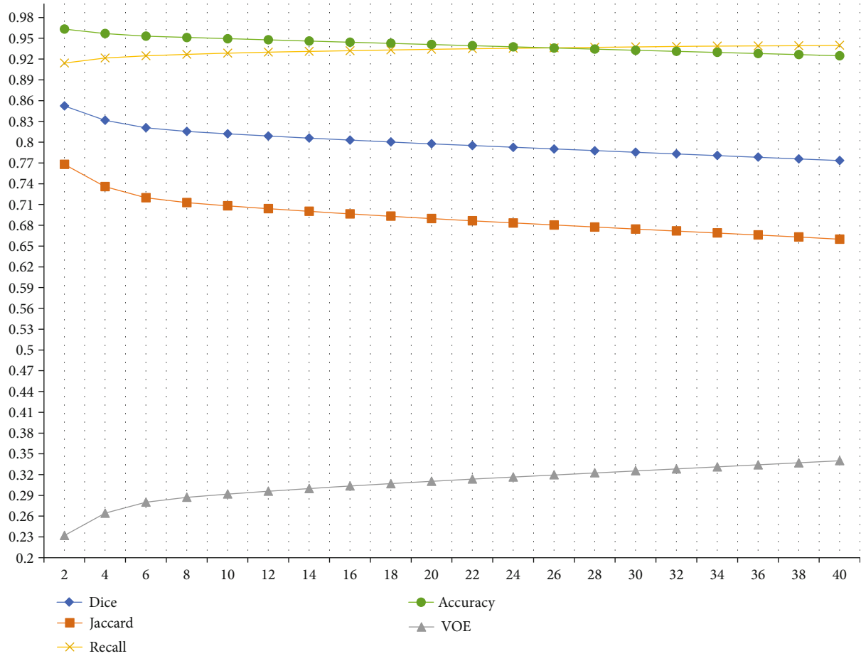
FIGURE 23: The evaluation indexes of the combined results under different buffers.
