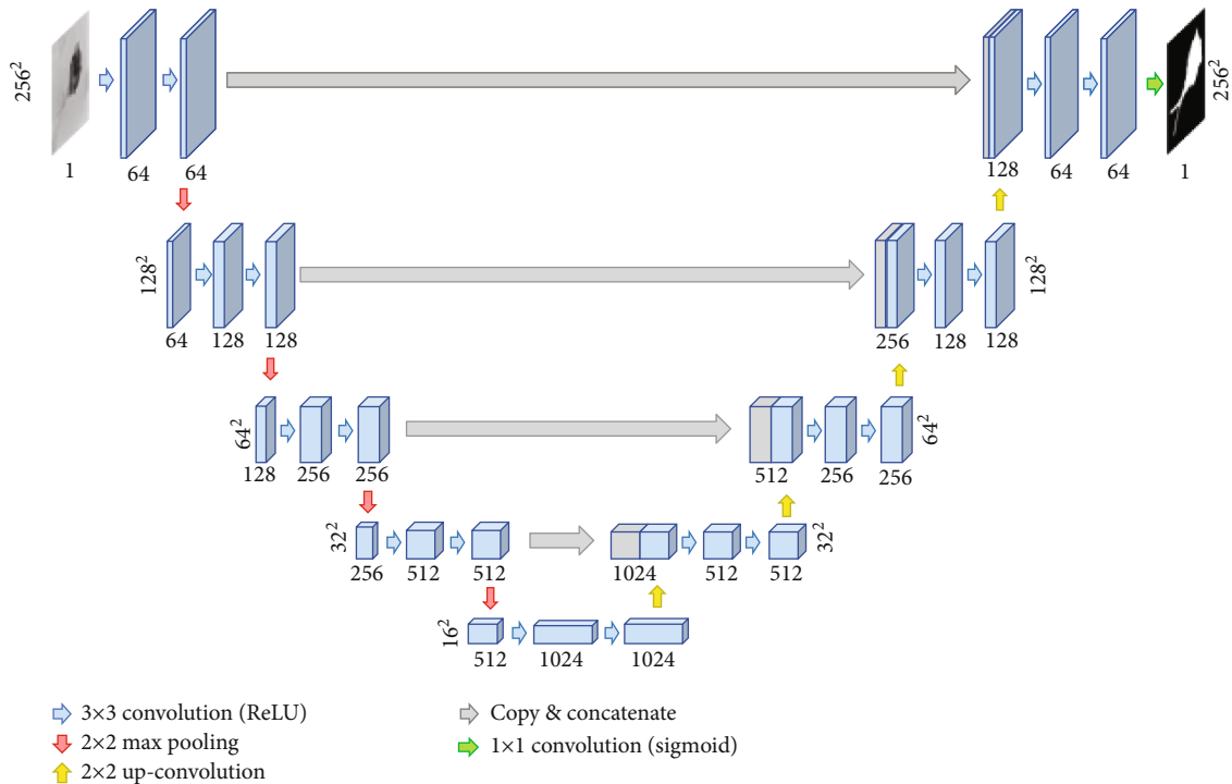
FIGURE 2: The network structure of U-Net.
