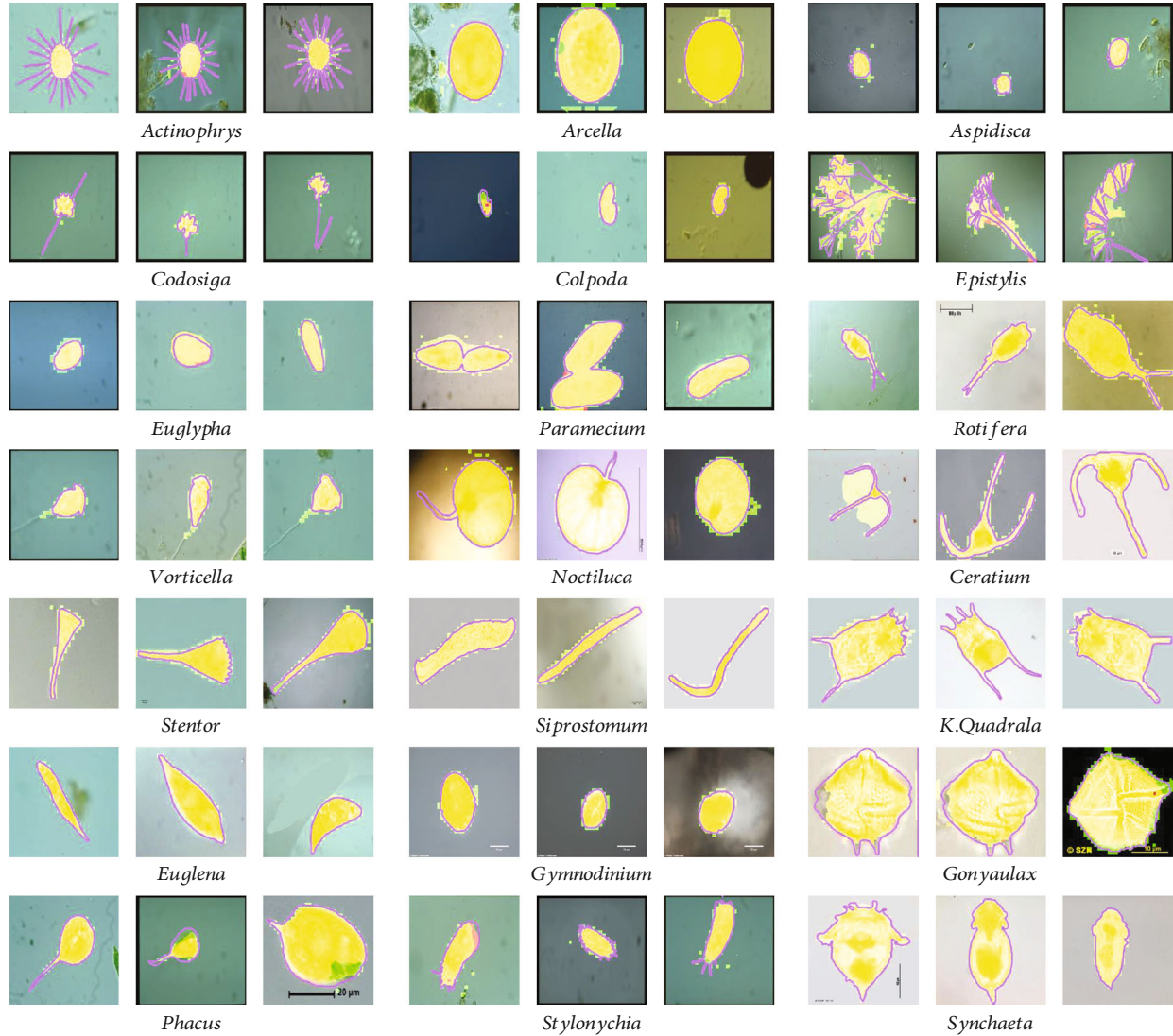
FIGURE 13: The combined results of pixel-level segmentation results and patch-level segmentation results. The red and fluorescent green masks represent pixel-level and patch-level segmentation results. The yellow masks represent the overlap of pixel-level and patch-level segmentation results. The purple outlines are the outlines of GT images.
