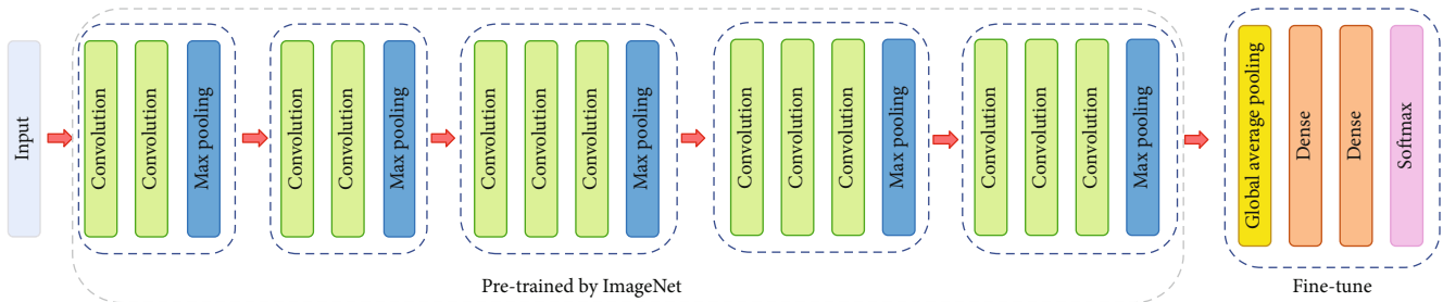
FIGURE 4: The architecture of VGG-16 network.
