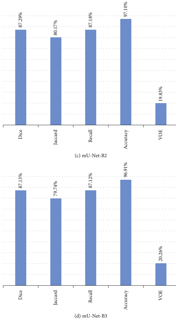
FIGURE 16: The average evaluation indexes of U-Net and mU-Net-BXs with denseCRF.
