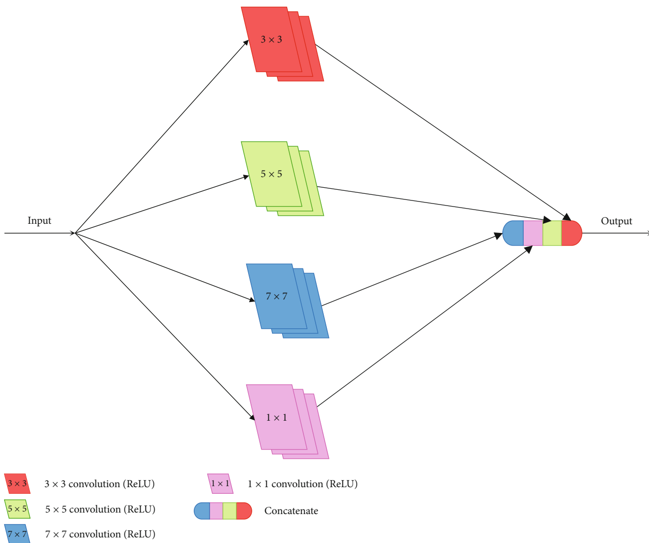
FIGURE 6: The architecture of BLOCK-I.
