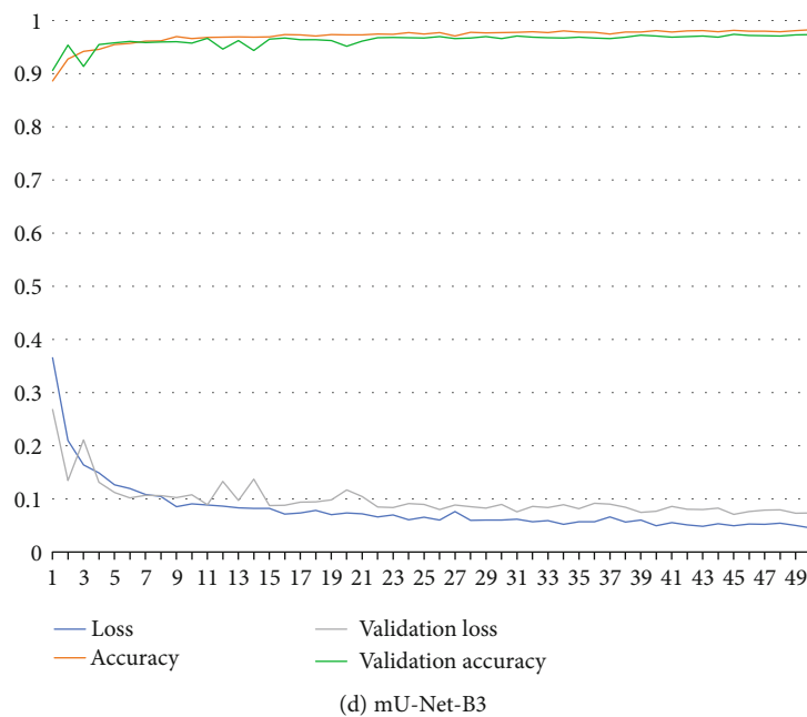
FIGURE 15: The loss and accuracy curves of the training process.
