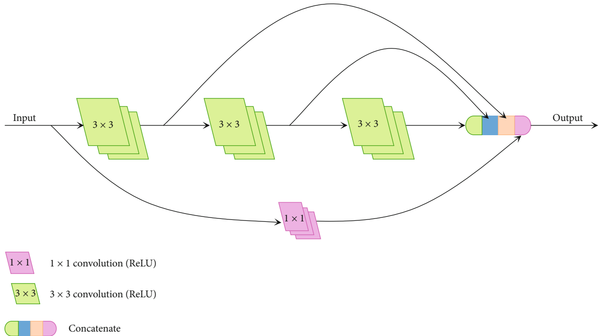
FIGURE 7: The architecture of BLOCK-II.
