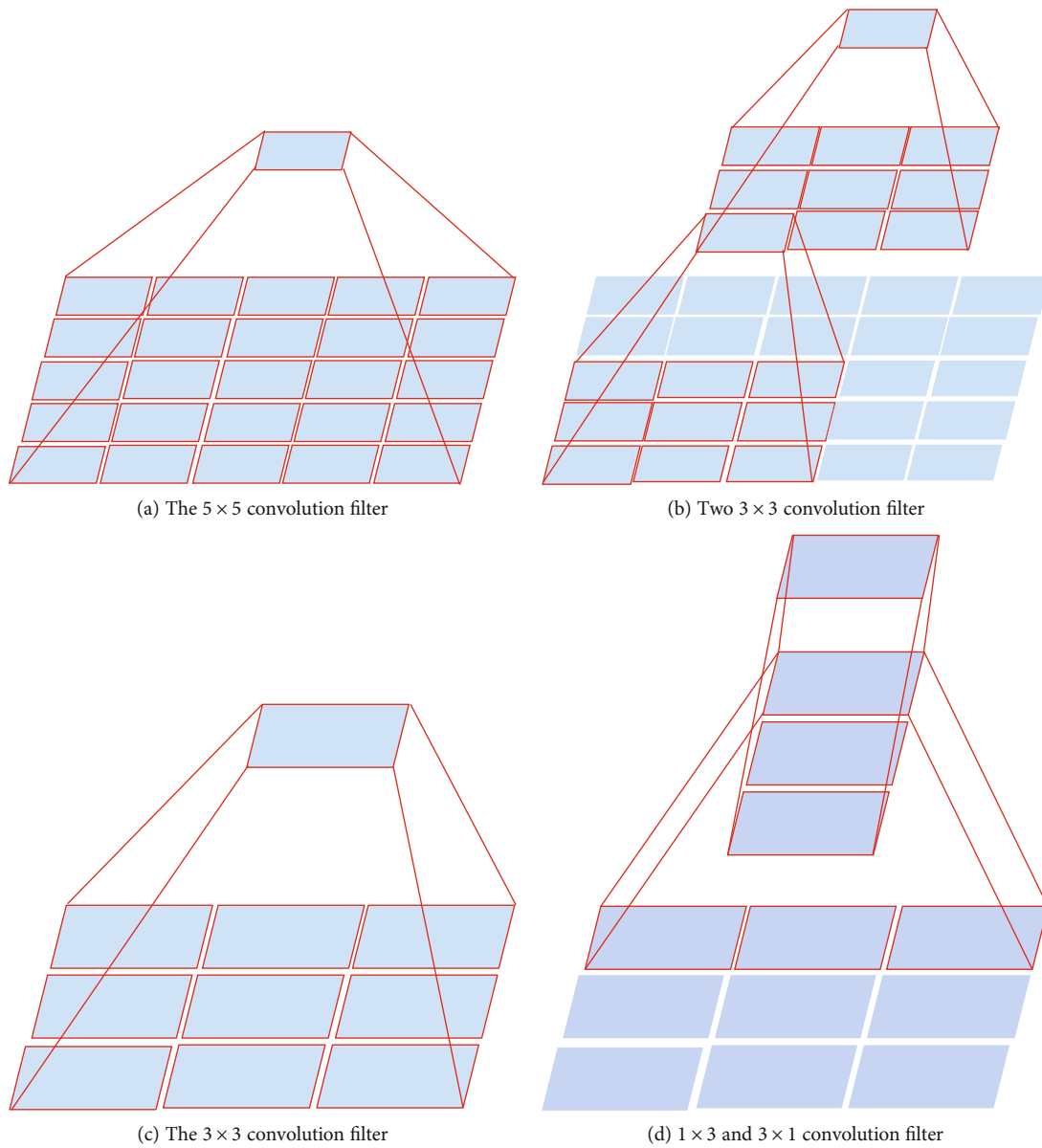
FIGURE 3: The strategies used by Inception-V2 and Inception-V3 to replace the big filter.
