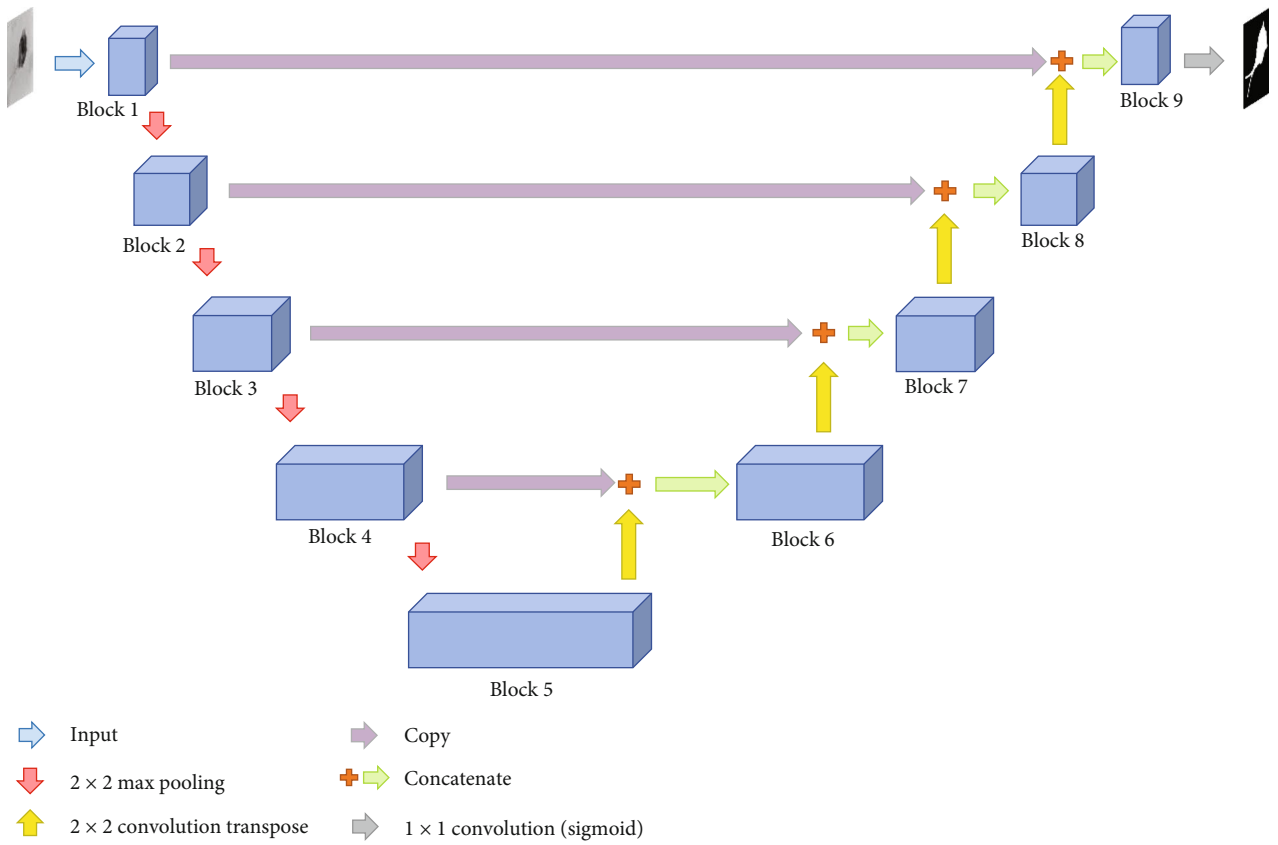
FIGURE 9: The architecture of mU-Net.
