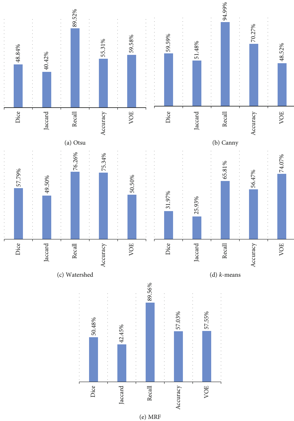
FIGURE 18: The average evaluation indexes of Otsu, Canny, Watershed, k -means, and MRF.
