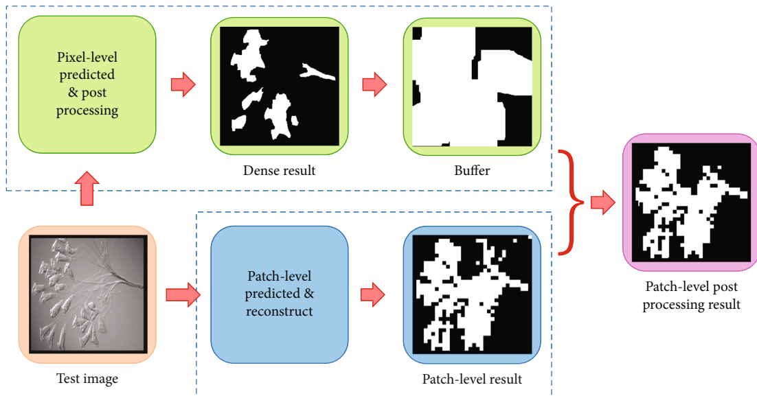
FIGURE 12: The workflow of the patch-level postprocessing.
