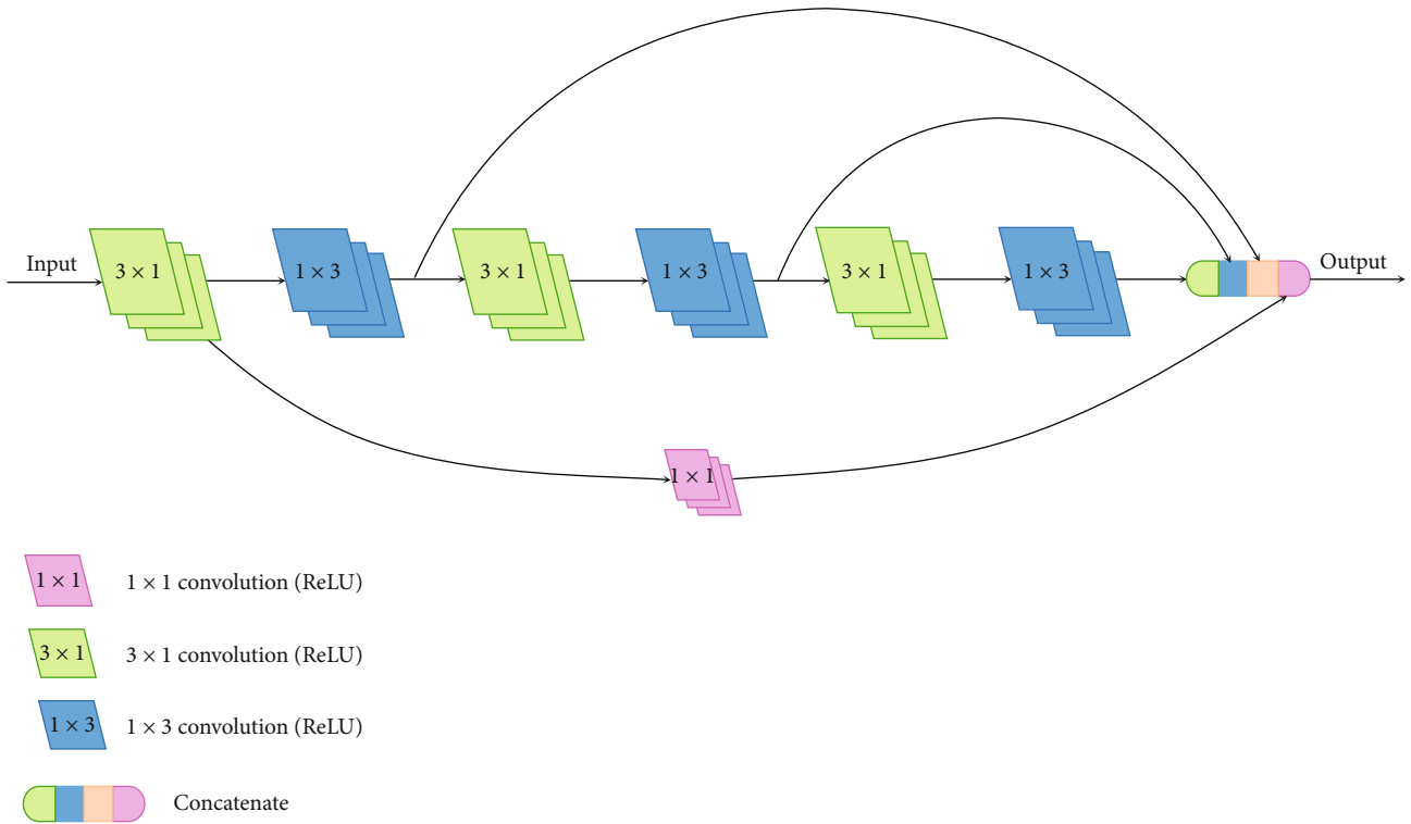
FIGURE 8: The architecture of BLOCK-III.
