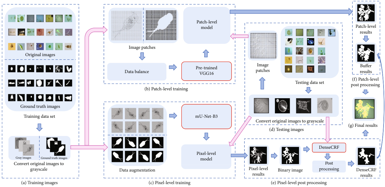
FIGURE 1: An overview of our MSCC EM segmentation framework.
