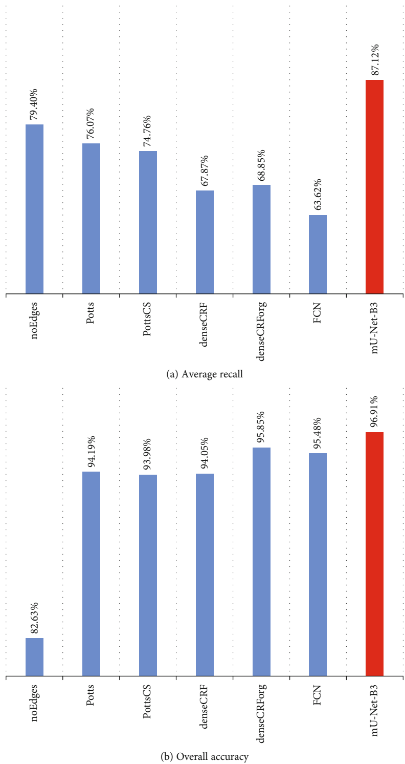
FIGURE 20: The average recall and overall accuracy of mU-Net-B3 with denseCRF and our previous models.
