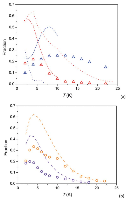
Fig. 5 Temperature dependence of susceptibility fractions F for relaxation paths SR1 and SR2 in 1 (a) and 2 (b) and related compounds. 1 – triangles, 2 – circles; colour designation for 1: red – SR2 and H = 8 kOe, blue – SR1 and H = 8 kOe; colour designation for 2: orange – SR2 and H = 8 kOe, violet – SR2 and H = 4 kOe. \text{Ca}_{9.5}\text{Tb}_{0.5}(\text{PO}_4)_6(\text{OH}_{0.75-\delta})_2 [ref. 29] (a) – short-dash lines; colour designation: red – SR2 and H = 4 kOe, blue – SR1 and H = 4 kOe, green – SR1 and H = 1.5 kOe. \text{Y}_{7.75}\text{Dy}_{0.25}\text{Ca}_2(\text{SiO}_4)_6\text{O}_2 [ref. 31] (a) – dotted lines; colour designation: red – SR2 and H = 4 kOe, blue – intermediate SR and H = 4 kOe. \text{Dy}_8\text{Ca}_2(\text{SiO}_4)_6\text{O}_2 , SR2 [ref. 31] (b) – dashed lines; colour designation: orange – H = 8 kOe, violet – H = 4 kOe.
