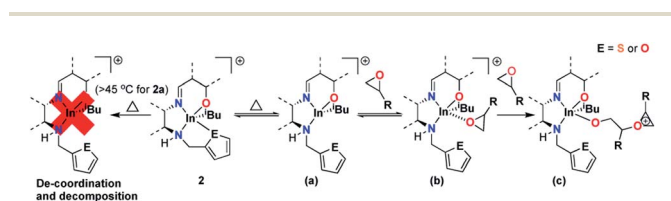
Scheme 2 Proposed behavior of cationic complexes with (a) increasing temperature, (b) in the presence of a low concentration of epoxide and (c) at high concentration of epoxide resulting in cationic polymerization.
