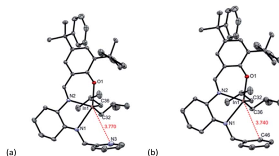
Fig. 1 Molecular structures of complex (a) [ L c ]In i Bu 2 ( 1c ) and (b) [ L d ]In i Bu 2 ( 1d ) (depicted with thermal ellipsoids at 50% probability and H atoms, as well as solvent molecules omitted for clarity).
