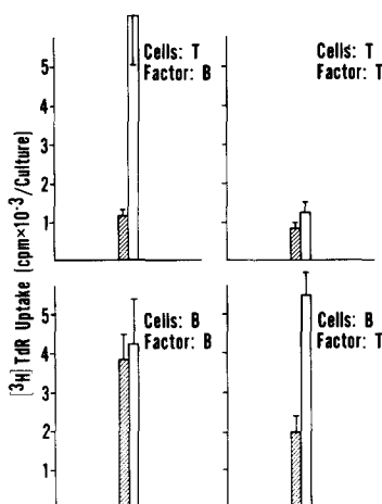
FIG. 7. Specificity of soluble factors isolated from B and T lymphocytes. 5 \times 10^5 viable C3H/St T or B lymphocytes were cultured for 2 d in 0.1 ml ( 5 \times 10^5 cell-equivalents) of 2-ME-induced or control soluble factor generated in cultures of B-cell-enriched or T-cell-enriched lymphocytes. Cells were pulsed with 1.0 \mu\text{Ci} of [^3\text{H}]\text{TdR} ( 6.7 \text{ Ci/mM} ) for the final 24 h of culture. Results are expressed as the arithmetic mean of nine replicate experiments \pm the standard error of the means. \square , control factor; \square , 2-ME-induced factor
