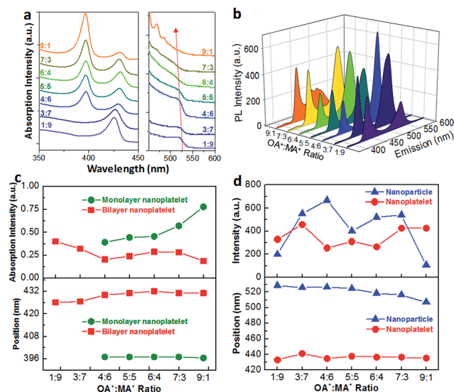
Fig. 5 Investigation of the impact of \text{OA}^+ : \text{MA}^+ ratios on the optical properties of the resulting \text{CH}_3\text{NH}_3\text{PbBr}_3 NCs solutions when using \text{PbBr}_2 + \text{Pb-oleate} as lead source. (a) UV-vis absorption curves of as-made \text{CH}_3\text{NH}_3\text{PbBr}_3 NCs solutions with varying \text{OA}^+ : \text{MA}^+ ratios. The curves were offset for better comparison. (b) PL emissions of as-made \text{CH}_3\text{NH}_3\text{PbBr}_3 NCs solutions with varying \text{OA}^+ : \text{MA}^+ ratios. The excitation wavelength was set as 350 nm. (c) The absorption peak intensity and position of mono- and bi-layer nanoplatelets from as-made \text{CH}_3\text{NH}_3\text{PbBr}_3 NCs solutions with varying \text{OA}^+ : \text{MA}^+ ratios. (d) The PL peak intensity and position of nanoplatelets and nanoparticles from as-made \text{CH}_3\text{NH}_3\text{PbBr}_3 NCs solutions with varying \text{OA}^+ : \text{MA}^+ ratios.
