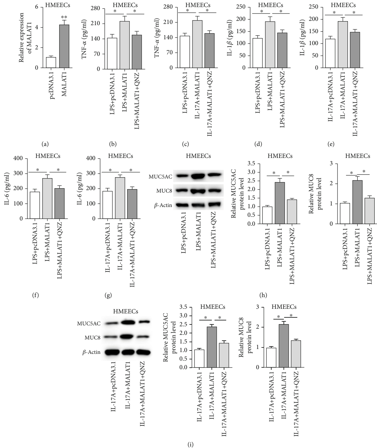
FIGURE 5: MALAT1 promotes LPS- or IL-17A-induced inflammatory response through the NF-κB pathway. (a) The overexpression efficacy of pcDNA3.1/MALAT1 in HMEECs was detected by RT-qPCR analysis. (b-g) The effects of MALAT1 and QNZ on concentrations of inflammatory cytokines (TNF-α, IL-β, and IL-6) were evaluated by ELISA assay in HMEECs under LPS or IL-17A treatment. (h, i) The effects of MALAT1 and QNZ on protein levels of MUC5AC and MUC8 were measured by western blot in LPS- or IL-17A-induced HMEECs. * p < 0.05, ** p < 0.01.
