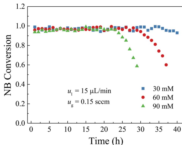
Fig. 8 Effect of the inlet nitrobenzene concentration on the NB conversion and durability.
