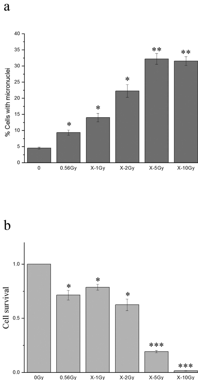
Figure 2. X-irradiation caused more serious damage and cell killing in directly irradiated HaCaT cells than 56Coγ of α-particles did. Panel a, the micronucleus formation in HaCaT cells 48h after irradiation. Panel b, the cell survival of irradiated HaCaT cells. * P < 0.05 , ** P < 0.01 , *** P < 0.001 compared with the sham irradiated control.
