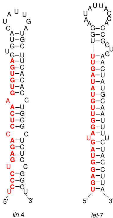
Fig. 1 The predicted stem loops for lin-4 (left) and let-7 (right). The sequences of mature miRNAs are shown in red.
