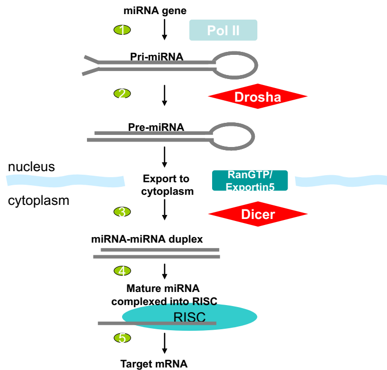
Fig. 2 Model of miRNA biogenesis.
