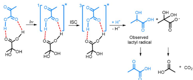
Scheme 1 Photo-decarboxylation of PA-PA H pair by UV-vis light. Dashed lines represent the hydrogen bonds between the PA and PA H . ISC represents the intersystem crossing mechanism by which the triplet state 3 [PA]* is created. 8,18,38
