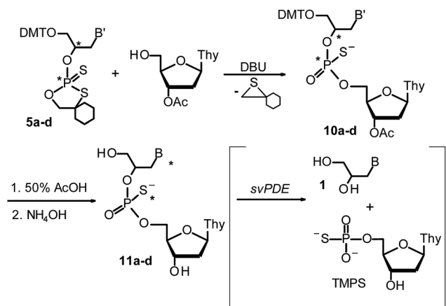
Scheme 4 Synthesis of "dinucleotides" {}^G\text{N}_{\text{PS}}\text{T} ( 11a-d ) using \text{OTP-}{}^G\text{N}' ( 5a-d ) and products of their hydrolysis (if successful) with svPDE .
