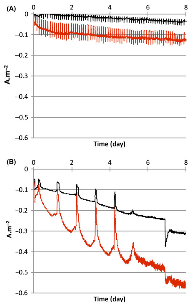
Fig. 2. Chronoamperograms of 3 cm 2 pre-colonized carbon felt biocathodes. Sulfur (A) or ferrous iron (B) was used as the prior energy source, either with C14-AHLs (red lines) or without C14-AHLs (black lines). CA was performed on MPG-2 potentiostat (Biologic) at E = -0.2 V versus Ag/AgCl KCl saturated reference and T = 30^{\circ}\text{C} .
