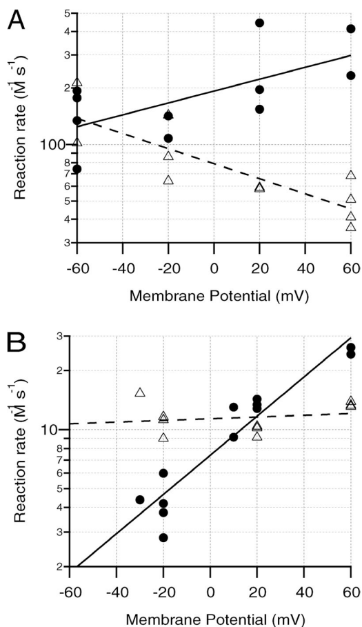
Figure 6. Estimation of MTS-ET reaction rates at 0 mV. (A) S305C. (B) S312C. Each graph is a semilog plot of the second-order rate constant, k , for cis ( \bullet ) or trans ( \Delta ) MTS-ET reaction versus voltage. Each data point represents one experiment. Linear fits of \log(k) versus voltage are shown. Interpolating to 0 mV gives k_{\text{cis}}/k_{\text{trans}} \approx 2.4 for S305C and 0.7 for S312C. Solutions were as in Fig. 2, except that for A, the buffers were 30 mM MES, pH 5.3 (cis), versus 50 mM HEPES, pH 7.2 (trans).
