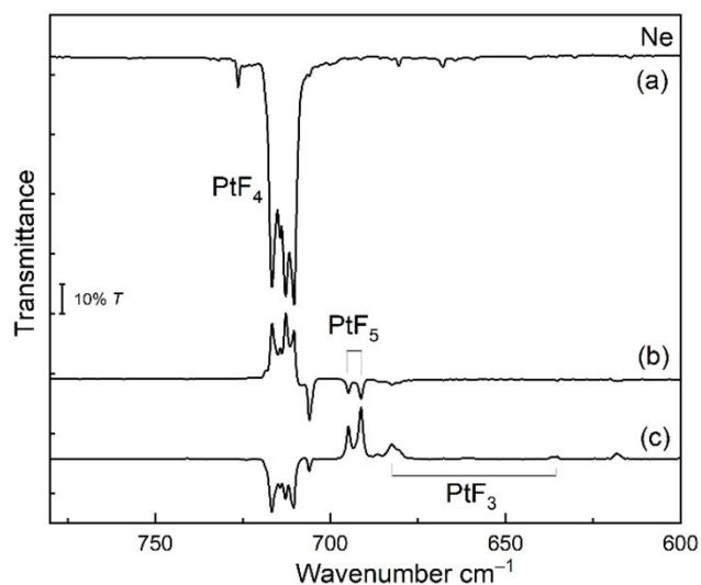
Figure 6. Infrared matrix-isolation spectra obtained in solid neon at 6 K. a) IR recorded after \lambda = 470 nm (blue LED) irradiation of the initial deposit of the PtF_6 precursor seeded in excess Ne. The difference spectra (b) and (c) show spectral changes obtained after \lambda = 266 nm (UV laser) irradiation for 60 min and subsequent \lambda = 375 nm (UV LED) irradiation for 80 min, respectively. Downward-pointing bands in the difference spectra are formed at the expense of upward-pointing bands.
