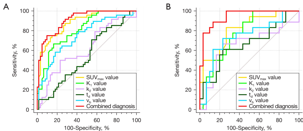
Figure 4 Curves show SUV max , K 1 , k 2 , t d , v b , and the combination of independent predictors by using receiver operating characteristic analysis for (A) differentiation benign and malignant pulmonary lesions and (B) differentiation of adenocarcinoma and squamous cell carcinoma. Details of the area under the curves and 95% CIs of each index are shown in the Results section and Table 4. SUV max , maximum standardized uptake value; K 1 , the forward transport rates of 18 F-FDG from plasma to tissue; k 2 , the backward transport rates of 18 F-FDG from plasma to tissue; v b , the blood fraction in the tissue; t d , the voxel-dependent delay time.
