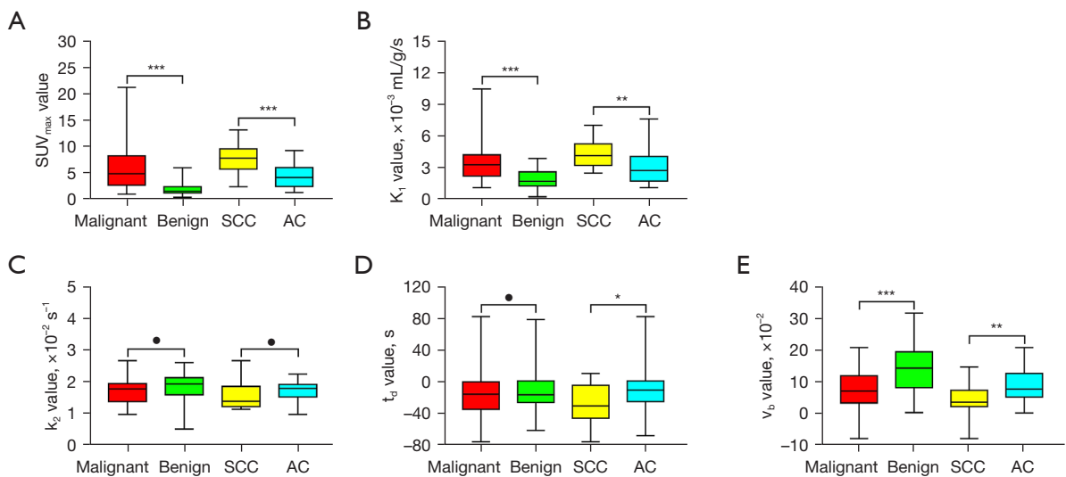
Figure 3 Box plot of different parameters. (A-E) represent SUV max , K 1 , k 2 , t d , and v b , respectively. *, P<0.05; **, P<0.01; ***, P<0.001; •, P>0.05. SUV max , maximum standardized uptake value; K 1 , the forward transport rates of 18 F-FDG from plasma to tissue; k 2 , the backward transport rates of 18 F-FDG from plasma to tissue; v b , the blood fraction in the tissue; t d , the voxel-dependent delay time.
