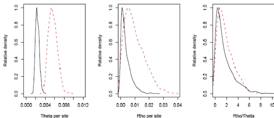
Figure 3 Posterior distributions of \theta , \rho and \rho/\theta as estimated using approximate Bayesian approach in foxtail millet (solid line) and green foxtail(dashed line).
