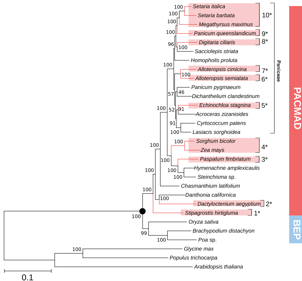
Fig. 1. Phylogenetic tree based on nuclear orthologs. C_4 taxa are in red, and C_4 origins are numbered. One of the tribe and the two main clades of grasses are indicated on the right. The black circle highlights the node representing the common ancestor of the sampled grasses. Bootstrap values are indicated near branches.
