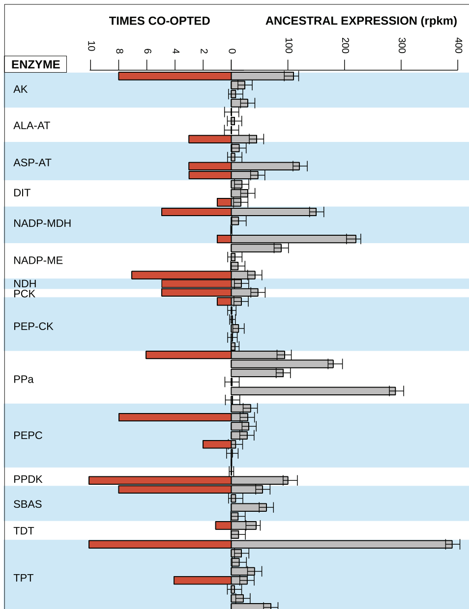
Fig. 4. Ancestral leaf transcript abundance and number of co-option events. Barplots on the left indicate the number of times each gene was co-opted, and those on the right indicate the inferred abundance in the non- C_4 last common ancestor of grasses (see fig. 1), with the associated confidence intervals. Genes are sorted by enzyme, indicated on the left.
