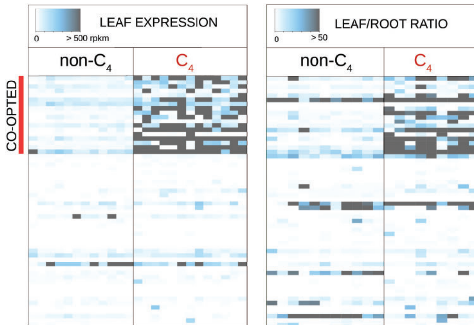
Fig. 3. Gene expression profiles of C_4 -related genes in the studied taxa. Colors indicate leaf transcript abundance and leaf/ratio abundance ratio for C_4 -related genes in C_4 and non- C_4 species. Genes that have been co-opted at least once are at the top.
