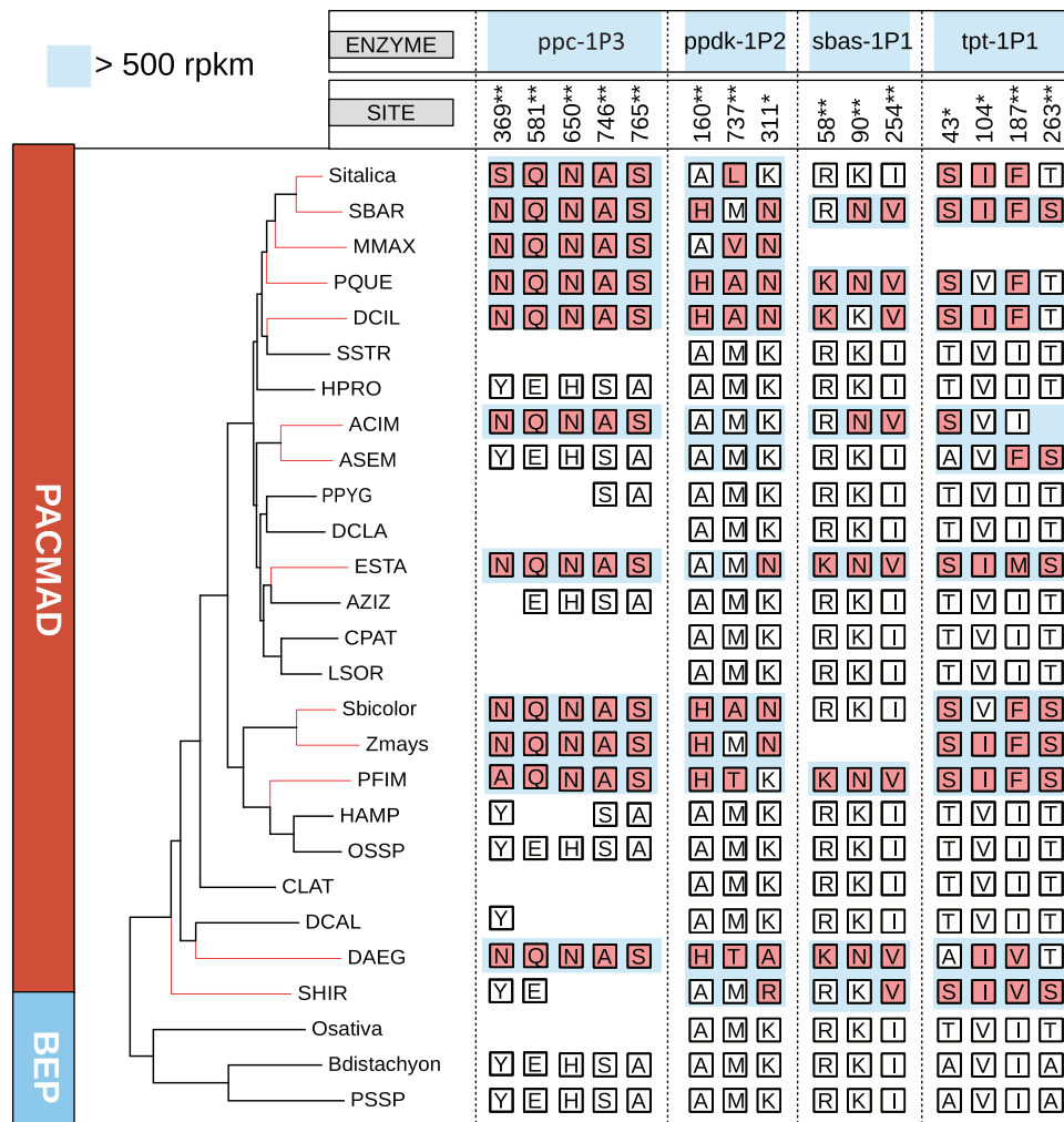
Fig. 5. Patterns of convergent adaptive amino acid replacements. The phylogeny of the sampled species is indicated on the left, with species names abbreviated as in supplementary table S1, Supplementary Material online. Branches leading to C_4 species in red. Amino acids at some of the sites under positive selection ( *P < 0.05 ; **P < 0.01 ) are indicated on the right. Residues of co-opted genes are highlighted with a blue background.
