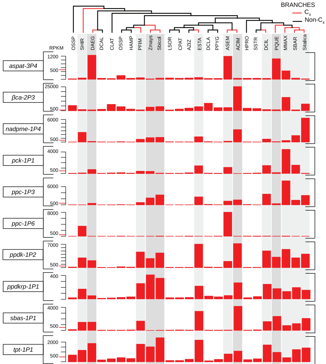
Fig. 2. Transcript abundances of the main C_4 genes in C_4 and non- C_4 species. Barplots indicate rpk values (reads per kilobase per million of reads). Phylogenetic relationships among species are indicated at the top, and C_4 lineages are numbered as in figure 1, with branches colored in red. Species names are abbreviated as in supplementary tables S1 and S2, Supplementary Material online.
