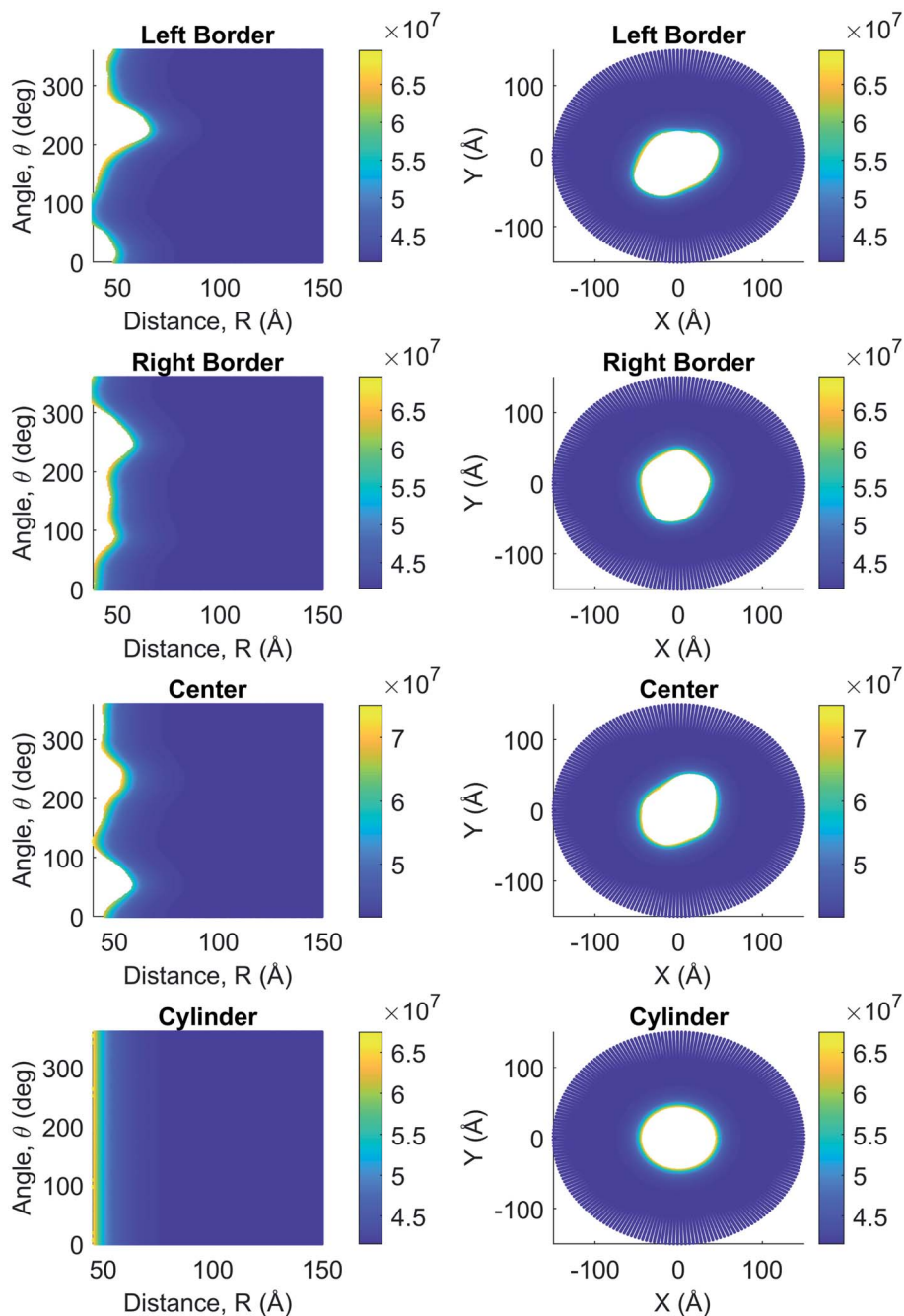
Fig. 11 In vitro longitudinal current density ( \text{A m}^{-2} ) as a function of angle, \theta ( ^{\circ} ), and separation distance, R ( \text{\AA} ), on the left column, and as cross-sectional views perpendicular to the filament's longitudinal axis on the right column. Both columns include data for the filament at the center, left, and right borders, as well as at the center of the cylinder model. The white space within the filament and cylinder (right column) is due to the transformation from cylindrical to Cartesian coordinates, as no data were taken inside the filament's domain.
