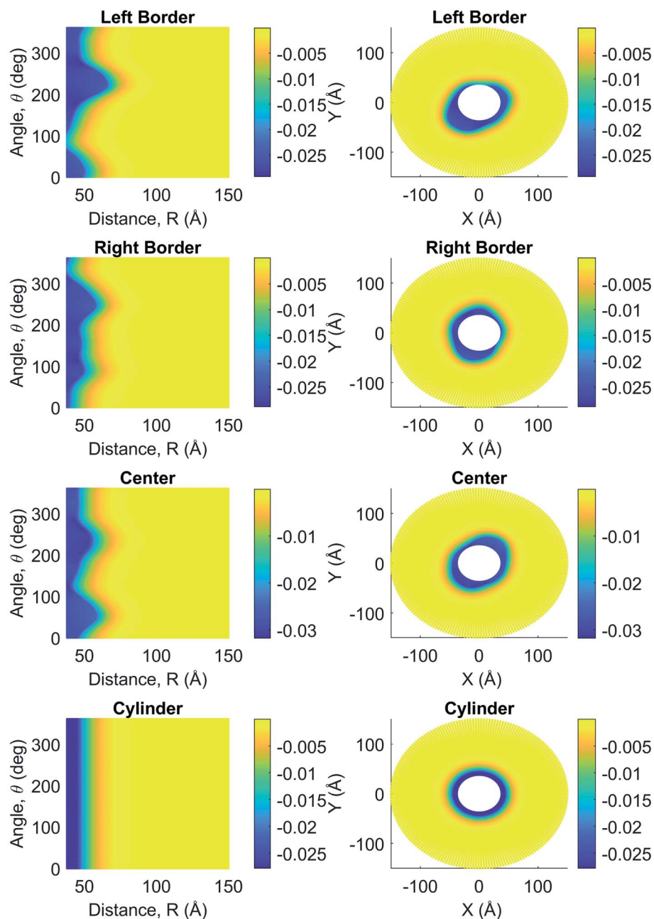
Fig. 3 Measurements for in vitro electric potential ( V ) as a function of angle, \theta ( ^{\circ} ), and separation distance, R ( \text{\AA} ), on the left column, and as cross-sectional views perpendicular to the filament's longitudinal axis on the right column. Both columns include measurements for the filament at the center, left, and right borders, as well as at the center of the cylinder model.
