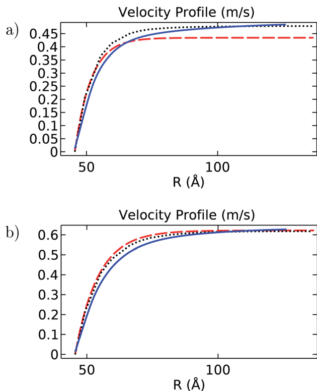
Fig. 8 Velocity profile ( \text{m s}^{-1} ) as a function of the separation distance R (Å) for (a) intracellular and (b) in vitro electrolyte solutions. In both graphs, the blue solid line is the angular average obtained for the filament, the black dotted line is the solution obtained for the cylinder model, and the red dashed line is the analytical solution.
