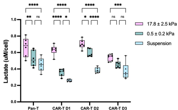
Fig. 4 Lactate production of Pan-T and CAR-T cells culture. Box plots show the means and SD of n = 6 samples after 5 days of culture. Statistical significance was calculated with two-way ANOVA and Tukey multi-comparison test. * P \leq 0.05 ; ** p \leq 0.01 ; *** p \leq 0.001 ; **** p \leq 0.0001 .
