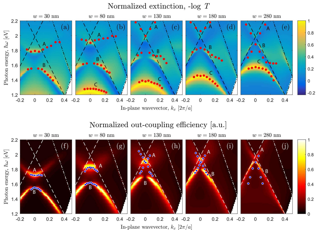
Figure 5. Extinction coefficient and out-coupling efficiency as functions of in-plane wavevector and photon energy. (a) Calculated k_x and energy dependencies of the extinction (panels (a)–(e)) and emissivity (panels (f)–(j)) spectra of the TM-polarized light for the sample with different air slit width. The magnitude of the extinction coefficient and emissivity is shown by different colors and the color scale is explained in color bars on the right. The red dots in panels (a)–(e) represent the experimentally observed extinction peaks, while the blue dots in panels (f)–(j) show the experimental PL peaks. The peak positions for the sample with 280 nm air slit are taken from ref. 23 .
