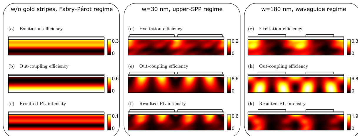
Figure 7. Spatial distributions of excitation efficiency, out-coupling efficiency and resulted PL intensity. Calculated excitation efficiency (a),(d),(g), outcoupling efficiency (b),(e),(h), and resulted PL intensity as a function of dipole position within the layer with silicon nanocrystals (c),(f),(k). The color scales of the corresponding quantities are shown in the color bars on the right. For comparison, the above quantities are shown for w = 0, 30 , and 180 nm. Quartz substrate is not shown in panels (a)–(k).
