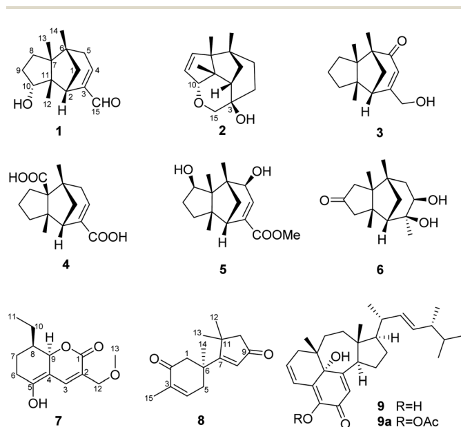
Fig. 1 Structures of compounds 1–9 , and 9a .
