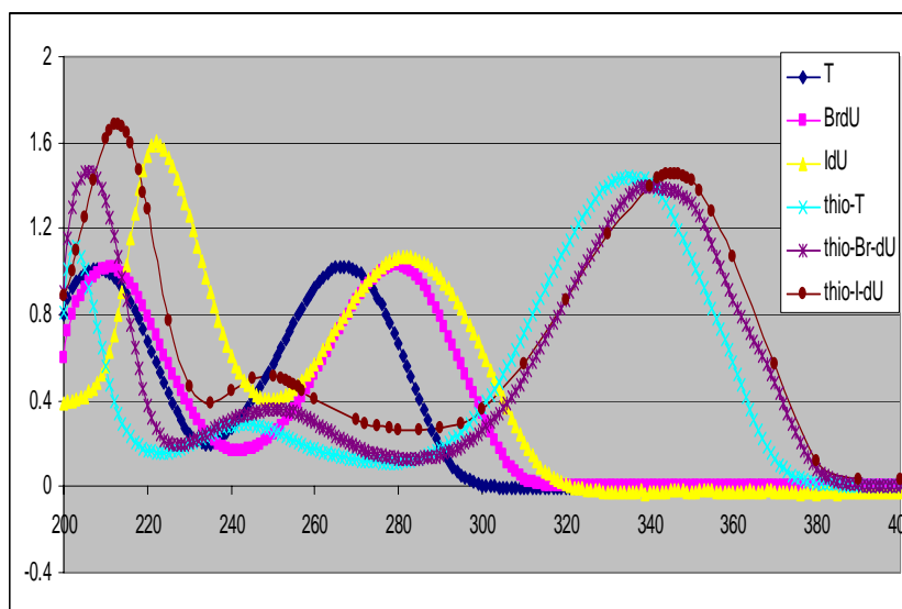
Figure 1. UV spectra of 5-substituted-2'-deoxyuridines (in CH 3 OH) and their 4-thioanalogues (in CH 3 CN).
