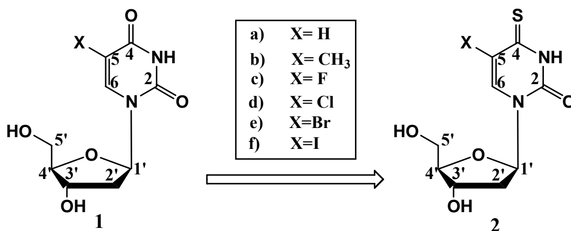
Scheme 1. Chemical transformation of 5-substituted nucleosides to its 4-thioanalogues.
