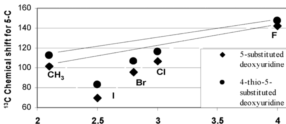
Figure 2. ^{13}\text{C} chemical shift of the atom (group) at 5-C plotted against its electro negativity.
