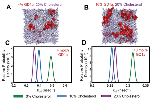
Fig. 3 Cholesterol slows GD1a–GD1a dissociation rates in molecular dynamics simulations. Simulation snapshots for membranes containing 20 mol% cholesterol and (A) 4 mol% GD1a or (B) 10 mol% GD1a. GD1a molecules showed reversible clustering in simulations containing 0, 10 or 20 mol% cholesterol. Cholesterol is rendered in purple, GD1a in red, and phospholipids in gray. (C and D) Probability density functions for GD1a–GD1a dissociation rate constants estimated from simulations. These compare rates over the range 0–20 mol% cholesterol at either 4 mol% or 10 mol% GD1a. Cholesterol significantly reduced k_{\text{off}} compared to sterol-free membranes under all of these conditions ( p < 10^{-6} ).
