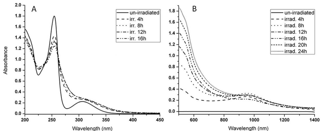
Figure 7. Absorption spectrum of 20 mg/mL of CPZ solution exposed to laser beam; beam energy at 266 nm is 6.5 mJ. A). Irradiation time up to 16 hrs; scanned from 200 to 500 nm. Sample diluted to 0.2 mg/mL after exposure. B). Irradiation time up to 24 hrs; scanned from 500 nm to 1500 nm 20 mg/mL. doi:10.1371/journal.pone.0055767.g007
