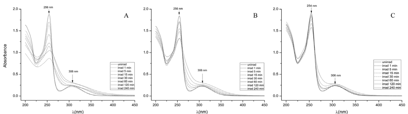
Figure 4. Absorption spectra of irradiated CPZ at concentrations of A) 5 mg/mL, B) 10 mg/mL and C) 20 mg/mL during 240 minutes. E=6.5 mJ. Note: After irradiation, an aliquot of the contents of the cuvette was diluted to 0.2 mg/mL and the shown absorption spectra were measured. doi:10.1371/journal.pone.0055767.g004
