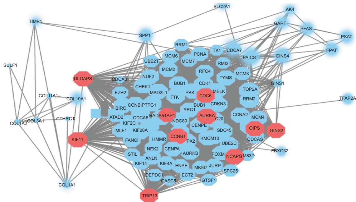
Figure 3 PPI of DEGs.
