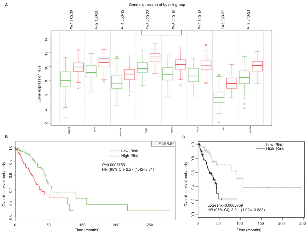
Figure 5 Prognostic gene signature of eight genes in LUAD patients of the TCGA cohort.
