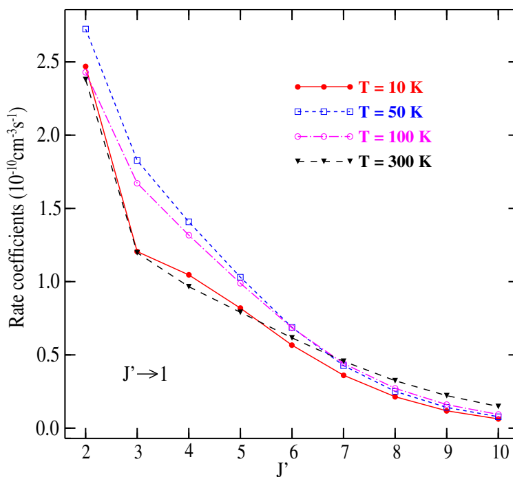
Figure 4 Calculated downward rate coefficients for the collisions of LiH with Ar for panel (a) J' \rightarrow 0 and panel (b) J' \rightarrow 1 transitions for selected kinetic temperature.
