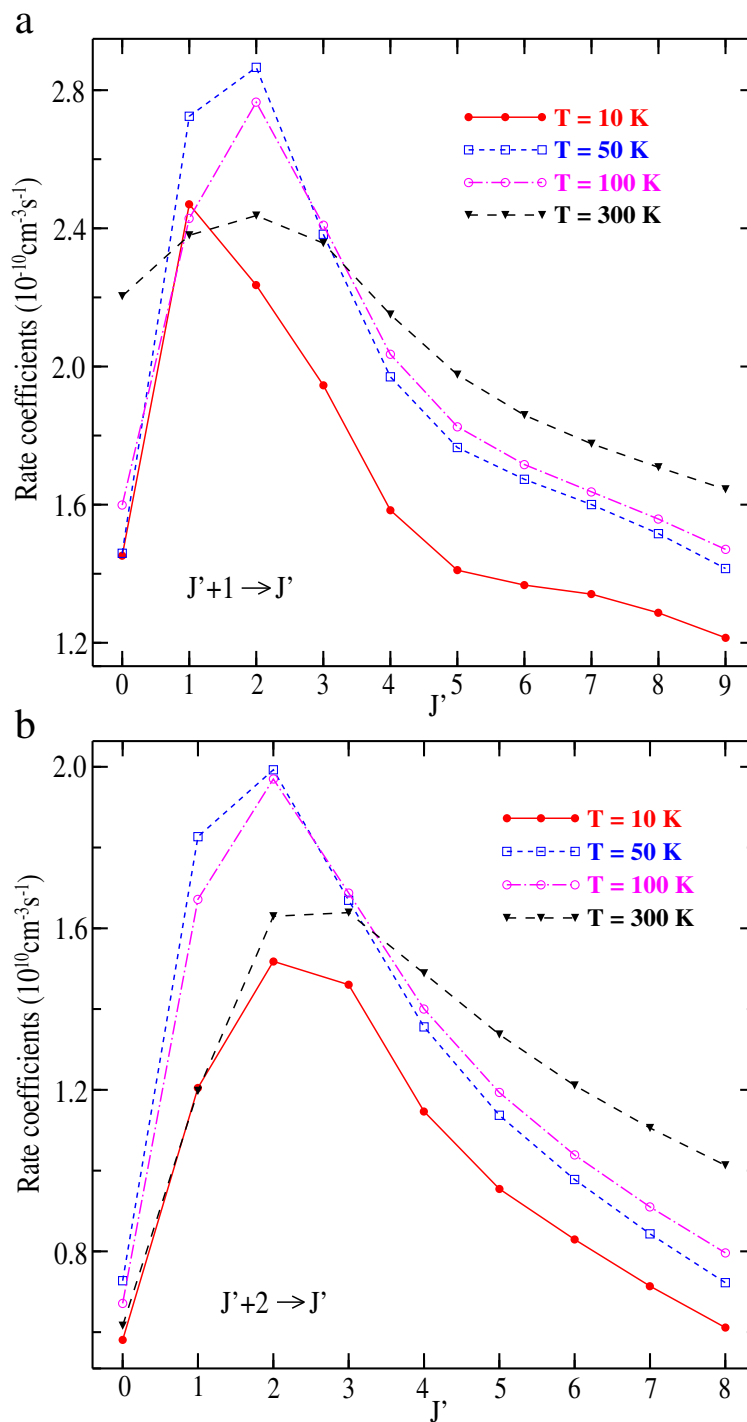
Figure 3 Calculated downward rate coefficients for the collisions of LiH with Ar for J'+1 \rightarrow J' and J'+2 \rightarrow J' transitions for selected kinetic temperature.
