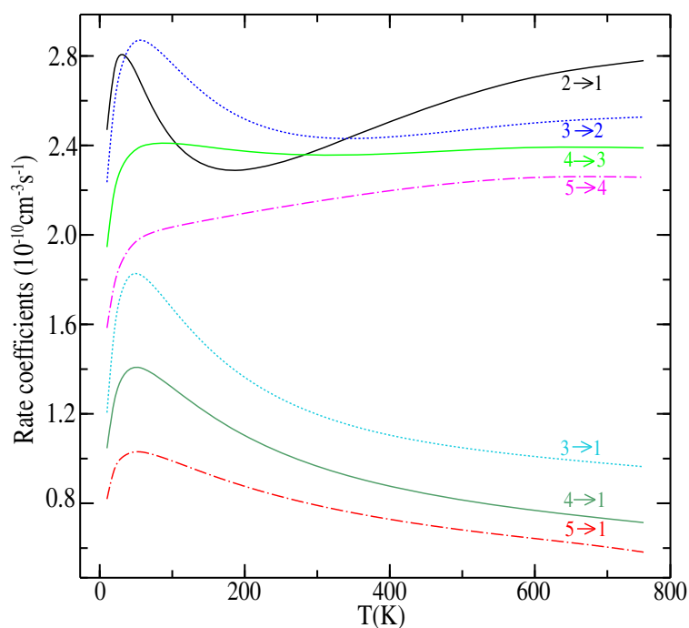
Figure 2 Calculated downward rate coefficients for the collisions of LiH with Ar for J \rightarrow 0 ( J = 2 - 5 ) panel (a) and \Delta J = -1 ( J' = 1 - 4 ; J = 2 - 5 ) and J \rightarrow 1 ( J = 2 - 5 ) panel (b) transitions as a function of the kinetic temperature.
