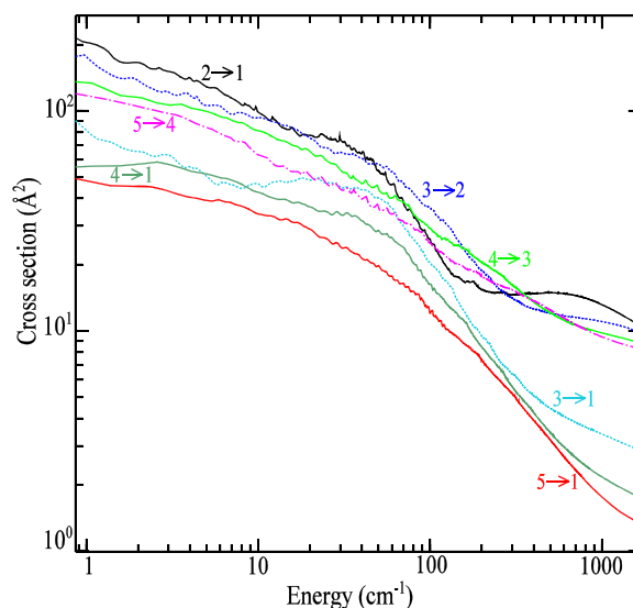
Figure 1 Rotational de-excitation cross sections of LiH in collision with Ar as a function of the relative kinetic energy.
