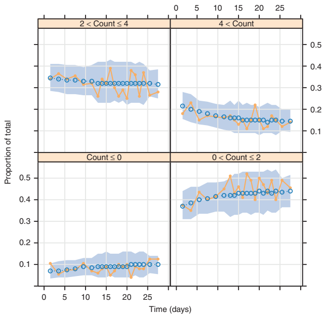
Figure 7 Visual predictive check for count data. Each panel represents the probability of observing a range of counts against time ( P(Y = 0) , P(1 \leq Y \leq 2) , P(3 \leq Y \leq 4) , P(Y \geq 5) ). The solid line is the median of the observed data and the ribbon the 95% confidence interval around the median (dotted line) of 500 simulations from a count model fitted to count data.
