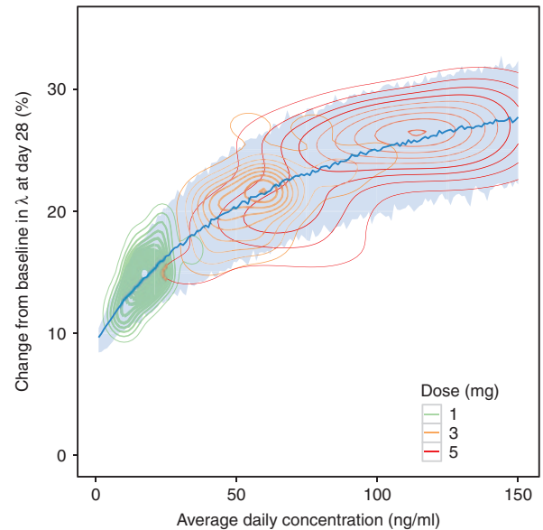
Figure 8 Dose selection plot. The exposure–response is depicted as change from baseline in \lambda at day 28 against average daily concentration. The blue elements are the model-based mean and 95% prediction interval generated from 500 simulations on a fine grid. The two-dimensional densities, built from patients observations, indicate the dose groups from the last conducted studies. A placebo group had been studied and a placebo effect observed.
