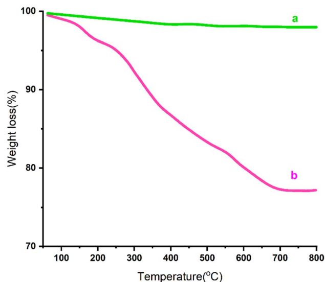
Fig. 5 TGA spectra of (a) \text{MCFe}_2\text{O}_4 and (b) \text{MCFe}_2\text{O}_4@ \text{Alginate}@ \text{SAA} .
