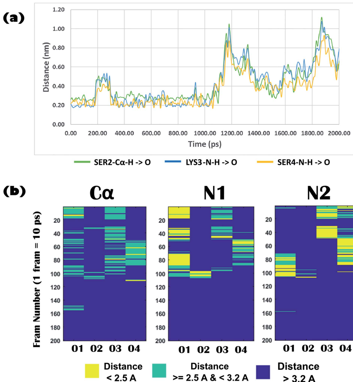
Fig. 5 (a) Time dependent variation of distance of the 'C \alpha NN' motif residues (C \alpha of Ser2, main-chain N-H of Lys3, main-chain N-H of Ser4) of DS3 and oxygen atoms of Arsenate ligand (HAsO _4^{2-} ). Up to 2 ns of the MD trajectory is shown in this figure where it can clearly be seen that the ion HAsO _4^{2-} interacts with the C \alpha NN region of DS3 up to 1.06 ns. (b) Distance profile of O atoms (up to 2 ns) of ligand (HAsO _4^{2-} ) from the Ser2-C \alpha -H, Lys3-N1-H, and Ser4-N2-H of 'C \alpha NN' motif residues of DS3 in time dependent manner resembling the C \alpha NN-HPO _4^{2-} interaction as reported in literature [X axis: oxygen atom number of the ligand HAsO _4^{2-} ; Y axis: frame number (1 frame = 10 ps, i.e. , up to 2000 ps to 2 ns is shown)].
