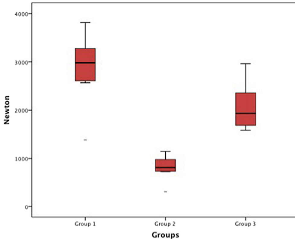
Fig. 3. Biomechanical test results.
