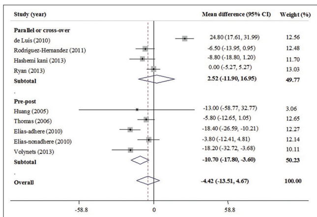
Supplementary Figure 1: Forest plot showing overall effect of low carbohydrate diet on serum alanine transaminase levels after removing ketogenic diets in subjects with nonalcoholic fatty liver disease and subgroup analysis based on study design (parallel or cross over and pre-post studies using random effects model)
