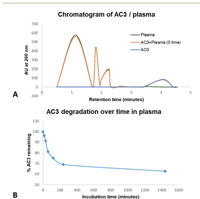
Fig. 3 Stability of AC3 in human plasma up to 24 hours monitored by HPLC-UV. (A) Comparison of human plasma elution time with AC3. (B) Degradation of AC3 in human plasma as a function of time.
