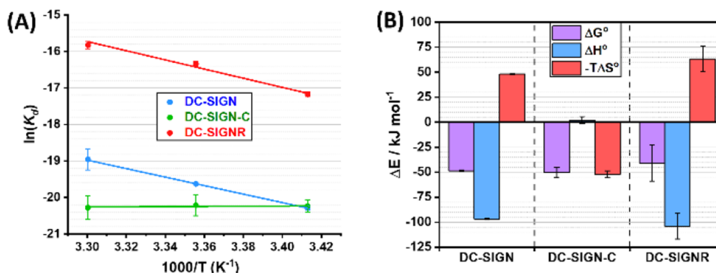
Figure 3. (A) Van't Hoff analyses of the \ln(K_d)-1/T relationships for QD-DiMan binding with DC-SIGN (blue), DC-SIGN-C (green), and DC-SIGNR (red). (B) Comparison of the standard ( T = 298 K) enthalpy (blue), entropy (red), and Gibbs free energy (pink) changes of QD-DiMan binding with DC-SIGN, DC-SIGN-C, and DC-SIGNR. SDs represent fitting errors.
