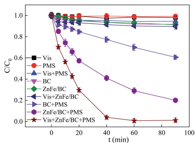
Fig. 5 Degradation of SDZ under different reaction conditions ( C_0 = 30 \text{ mg L}^{-1} , \text{pH} = 6 , \text{PMS} = 5 \text{ mmol L}^{-1} , \text{ZnFe/BC} = 0.5 \text{ g L}^{-1} , \lambda \geq 400 \text{ nm} ).
