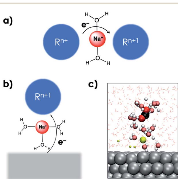
Fig. 5 (a) Schematic representation of alkali cation promoted outer-sphere ET between two species in the homogeneous phase. (b) Proposed schematic representation of alkali cation mediated outer-sphere ET from a cathode surface to a species in the homogeneous phase. (c) Snapshot of an AIMD trajectory with the \text{O}=\text{C}=\text{O} angle constrained at 140^\circ showing the interaction between a solvated cation in the EDL and the solvated \text{CO}_2 moiety analogous to the schematic depiction in (b). VdW representation is used for the \text{CO}_2 moiety interacting with a solvated \text{Na}^+ cation along with its first solvation shells which are shown in brushed metal colors. Other \text{Na}^+ cations are shown as smaller spheres, and water molecules are shown via line representation. Periodic images have also been included.
