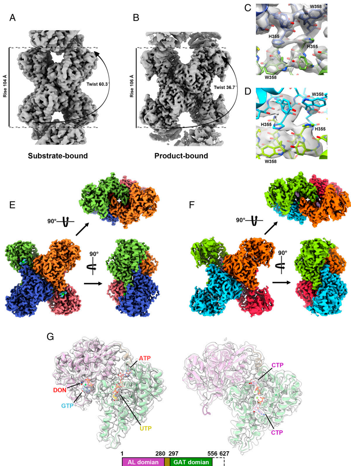
Fig. 1. Overall structures of substrate-bound and product-bound Drosophila CTPS tetramer. ( A and B ) Cryo-EM reconstructions of substrate-bound ( A , 2.48-Å resolution) and product-bound ( B , 2.65-Å resolution) dmCTPS tetramers. ( C and D ) The models and maps of the tetramer-tetramer interaction interface of substrate-bound ( C ) and product-bound ( D ) dmCTPS polymers. ( E and F ) Models of substrate-bound ( E ) and product-bound ( F ) dmCTPS tetramers. ( G ) Models of dmCTPS monomers display binding site of each ligand in substrate-bound and product-bound states. Residues 556-627 are disordered in the models.
