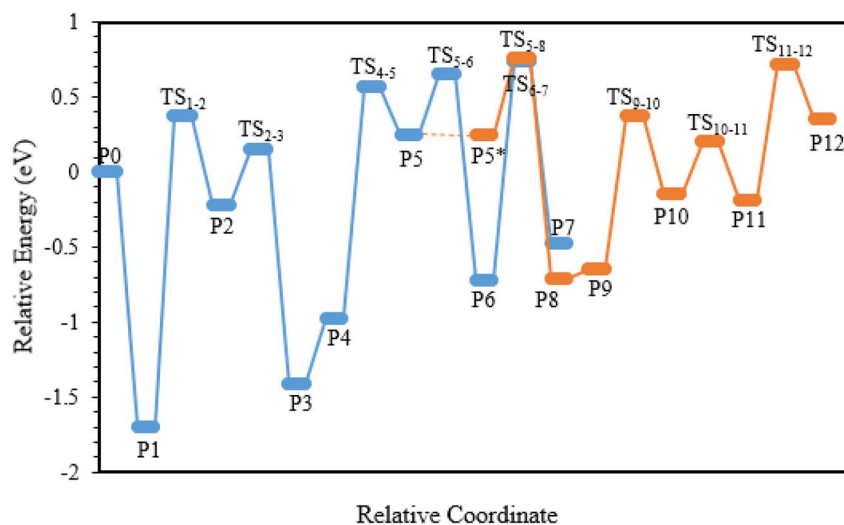
Fig. 7 Energy profile of the PX pathway in the side-chain hydrocarbon pool mechanism on Zr-ZH.
