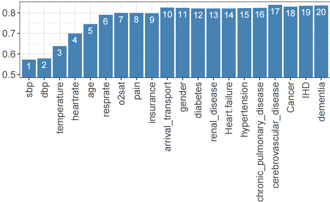
B Parsimony plot on the validation set
